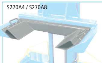
S270A4 / S270A8 S270A4 - Ø 800 ÷ 700 mm → max 7.500 kg S270A8 - Ø 700 ÷ 500 mm → max 7.500 kg
